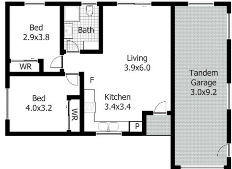
GRANNY FLAT
