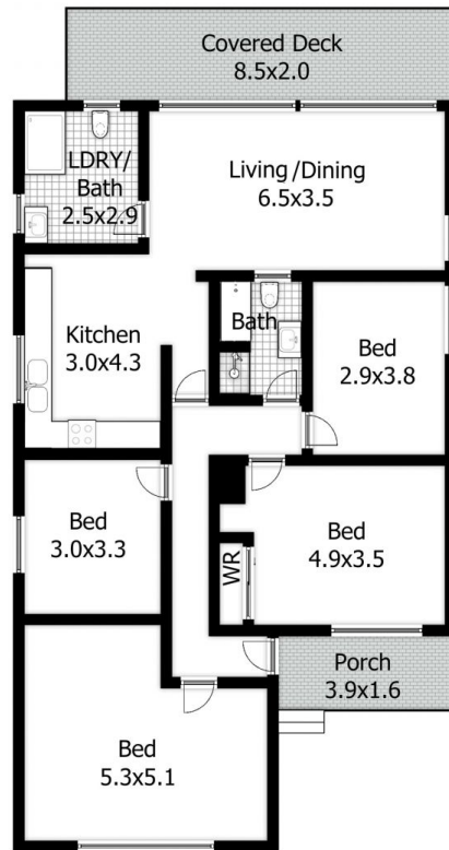
FLOOR PLAN
